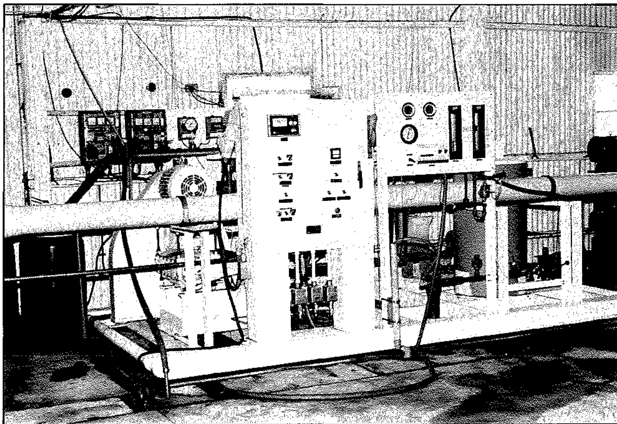
A reverse osmosis unit which is used at Swakopmund in the research on the desalination of sea water
