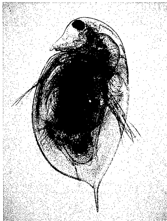
Right: The Daphnia pulex used for lethality tests
