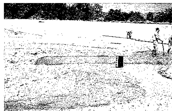
Olifants River at Barandas: These photos show the problems experienced at the gauging weir as a result of high sediment levels in the pool. The pool must be cleaned regularly to enable meaningful measurements to be made at the gauging weir
