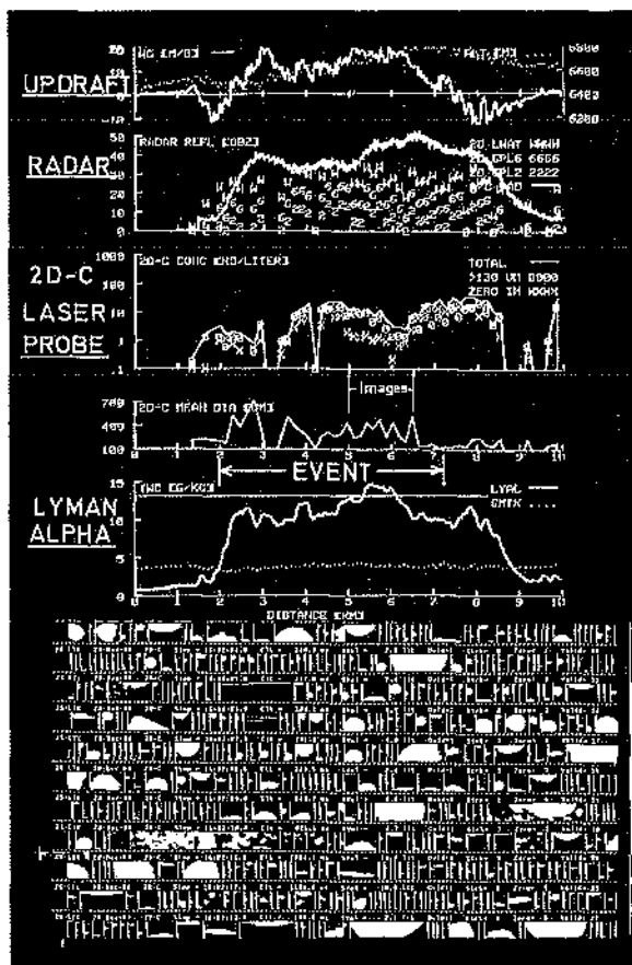
Display of cloud conditions and particle images on board the aircraft
