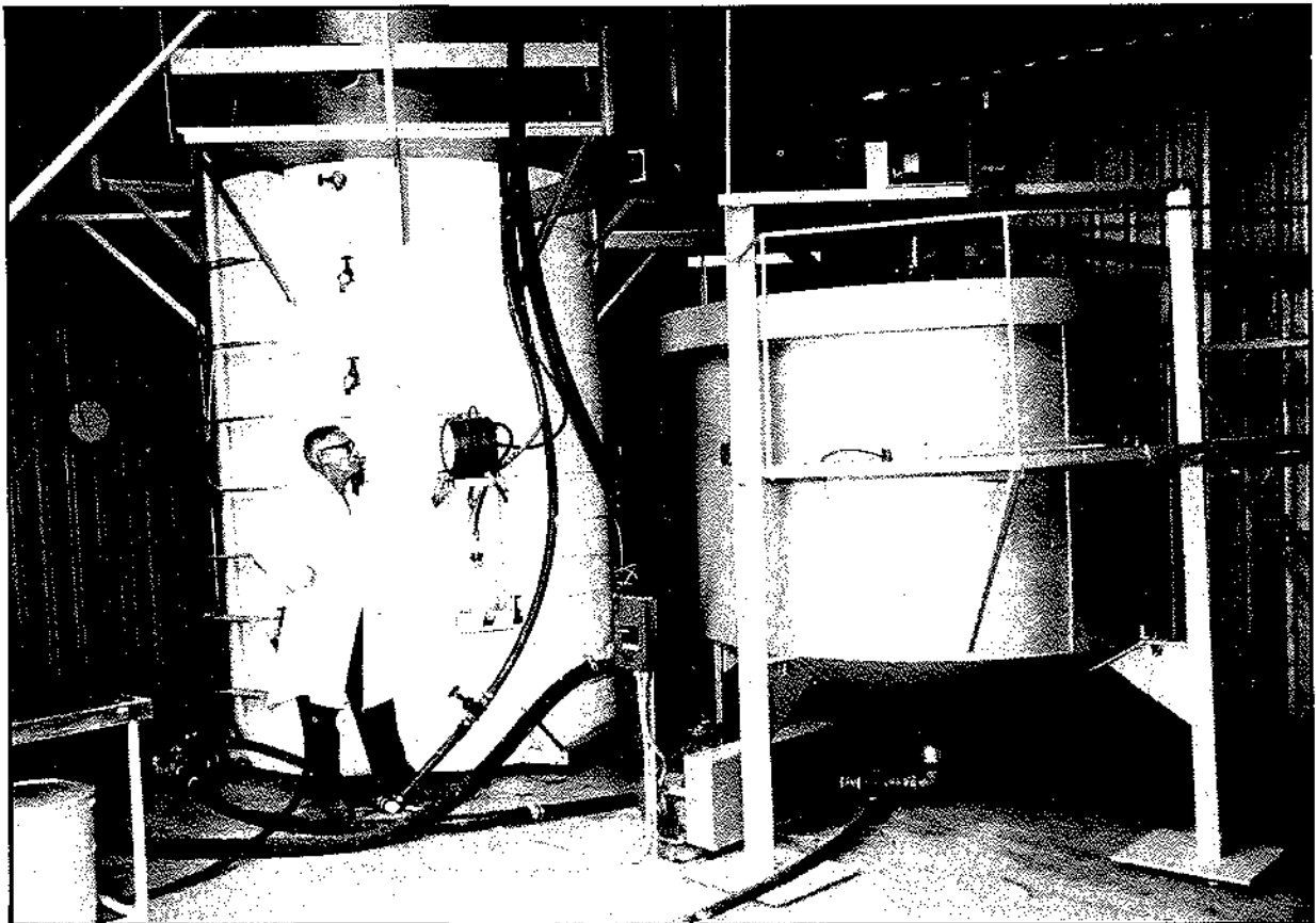
The pilot scale Clarigester of 7 \text{ m}^3 which is used in an experimental investigation into the treatment of spent wine effluents.
