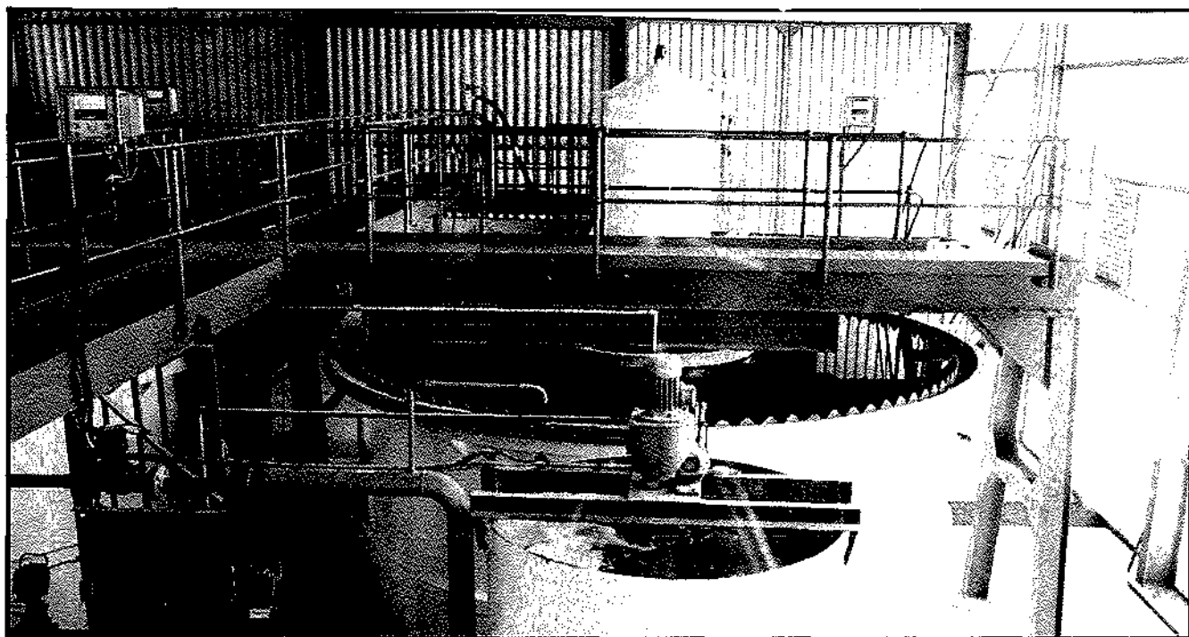
The lime reactor and primary clarifying process units at the Athlone Water Reclamation Plant.
