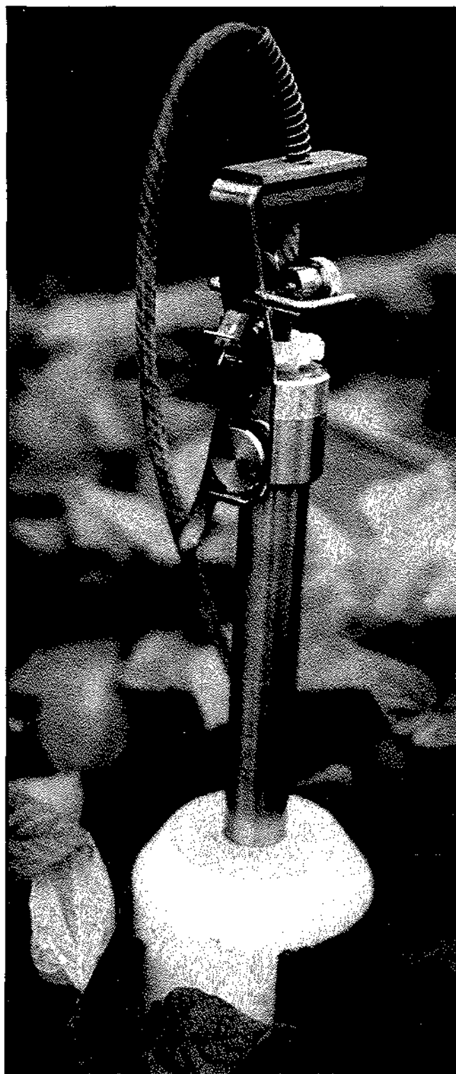
The probe of a neutron moisture meter with which soil moisture can be determined. This apparatus is used in determining the plant moisture stresses on the growth and production of certain agronomic crops.
