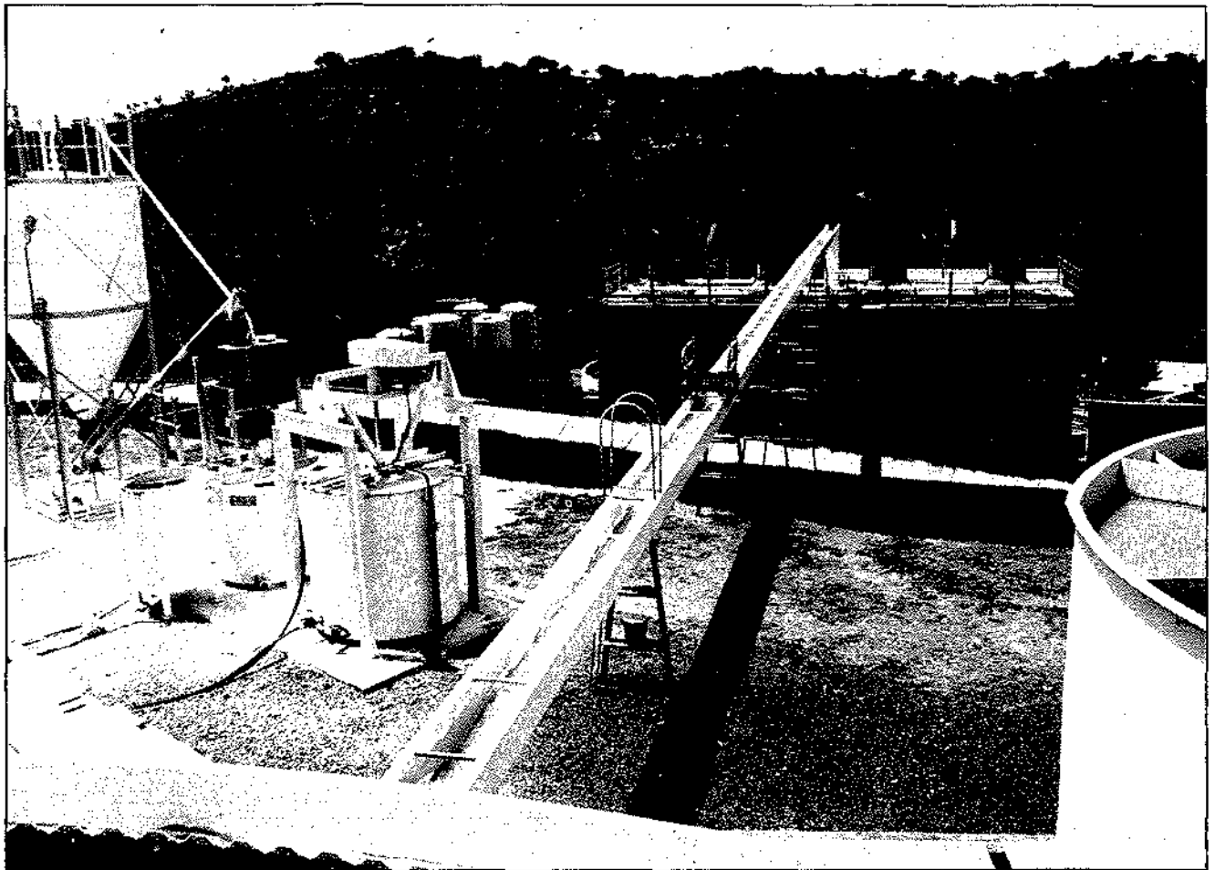
A part of the Windhoek Water Reclamation Plant which continues to play an important role in the city's water supply. The conduit (centre) leads from the primary sedimentation tank to the ammonia stripping tower. To the left (in the far background) the activated carbon columns, and on the extreme left the lime container may be seen.
