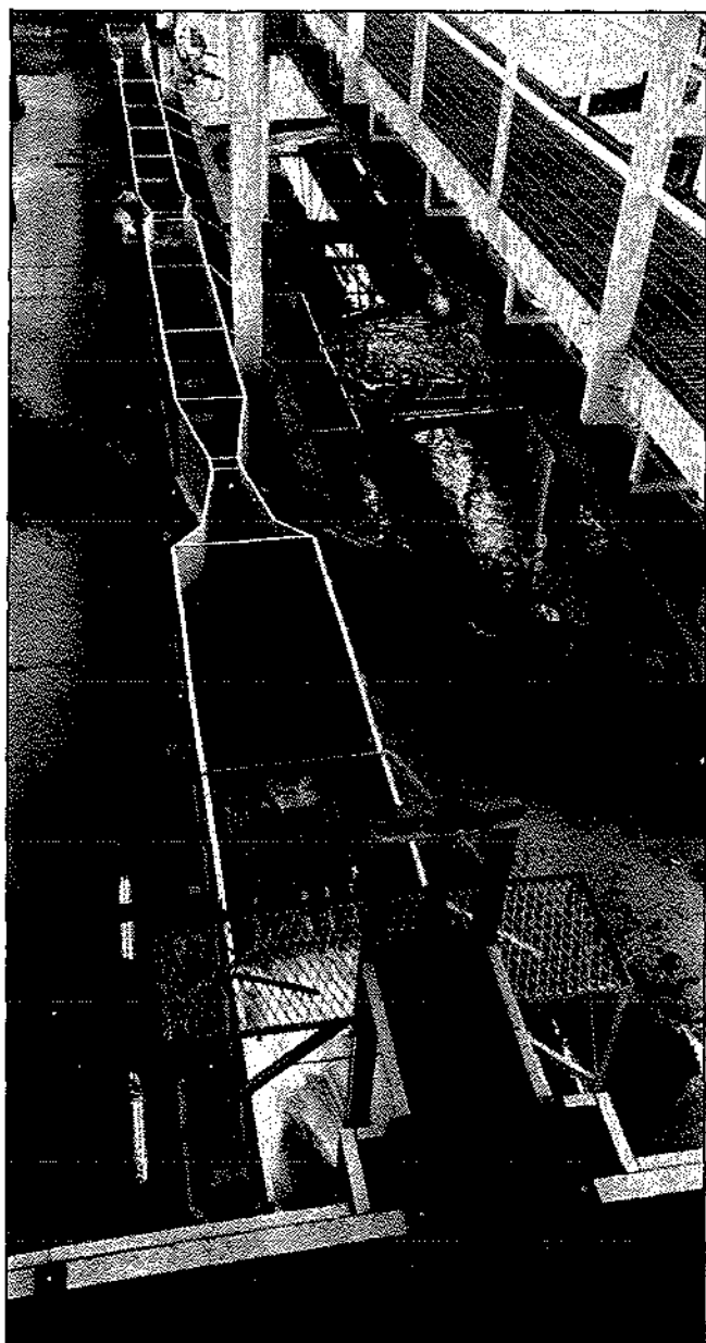
(Left) A variety of flumes in an open conduit at the Hydraulics Laboratory of the Department of Civil Engineering of the University of Stellenbosch. This equipment forms part of a project on the irrigation of steep lands.
