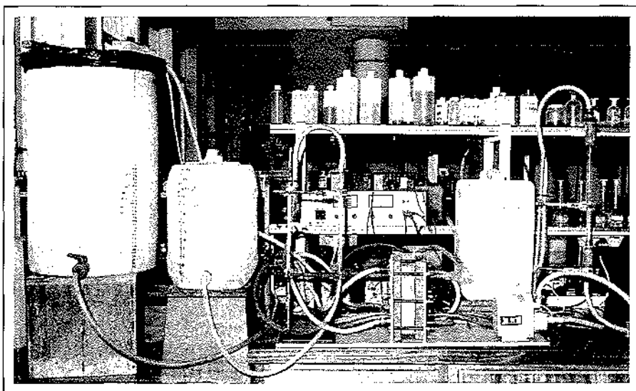
A bipolar electrodiolysis unit for the treatment of industrial effluents
